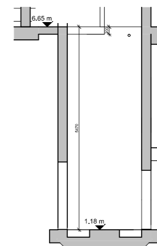
B12-5 Section B12 - 5 1 : 50
