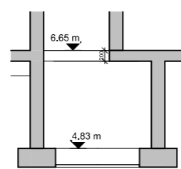
B12-2 Section B12 - 2 1 : 50
