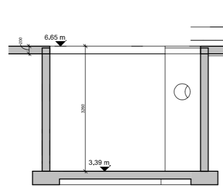
B12-3 Section B12 - 3 1 : 50
