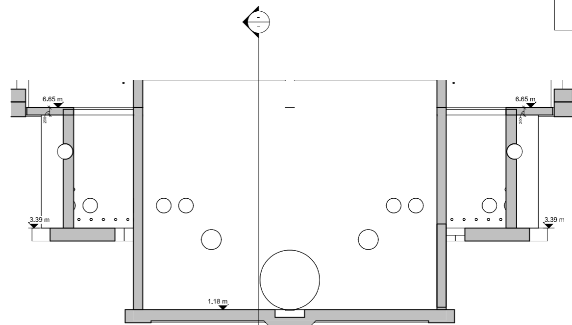
B12-3 Section B12 - 3 1 : 50
