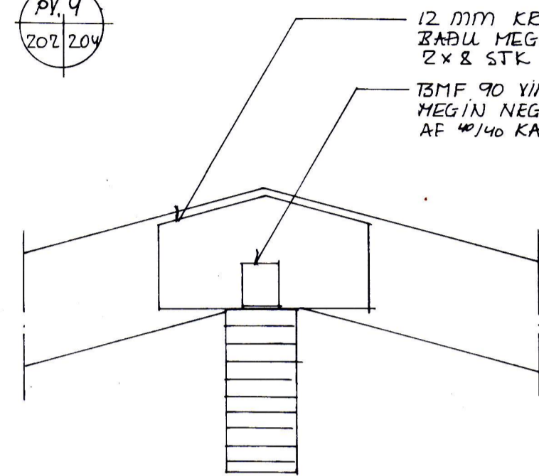
FESTING SPERU VÍÐ LIMTRÉ M=1:10
