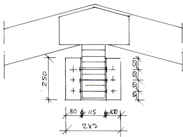
FESTING LIMTRÉ M=1:10
