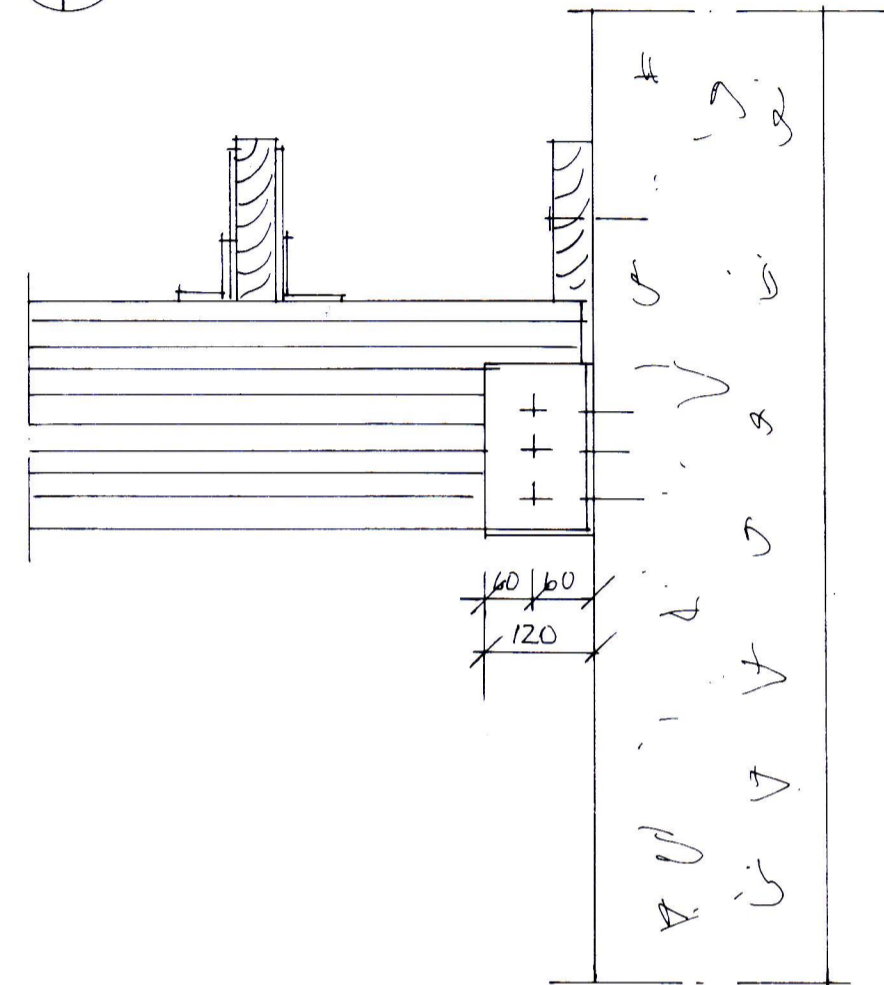
FESTING LIMTRÉ M=1:10
