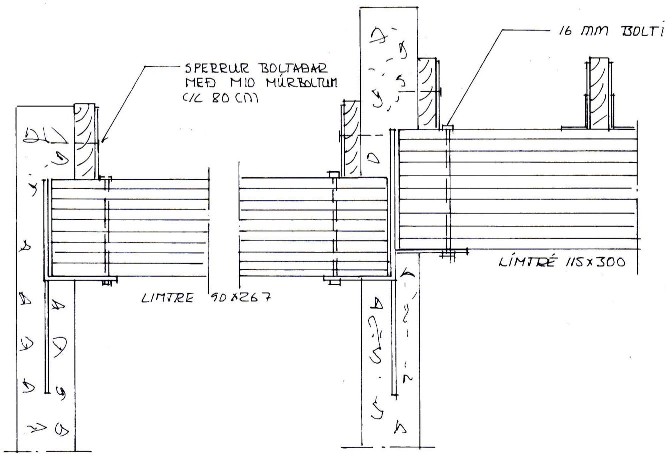
FESTING LIMTRÉ M=1:10
