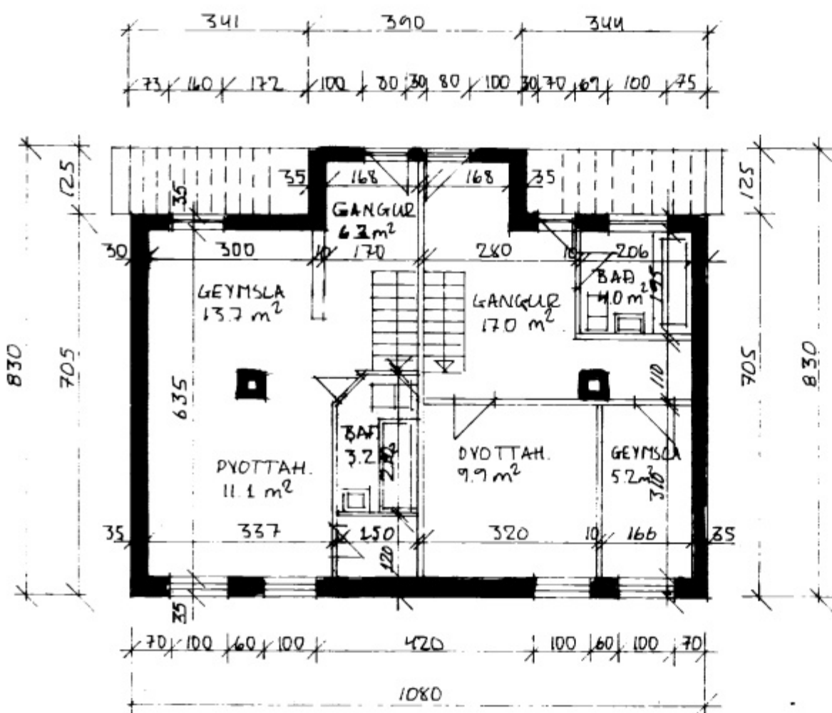
KJALLARI MKV 1:100
