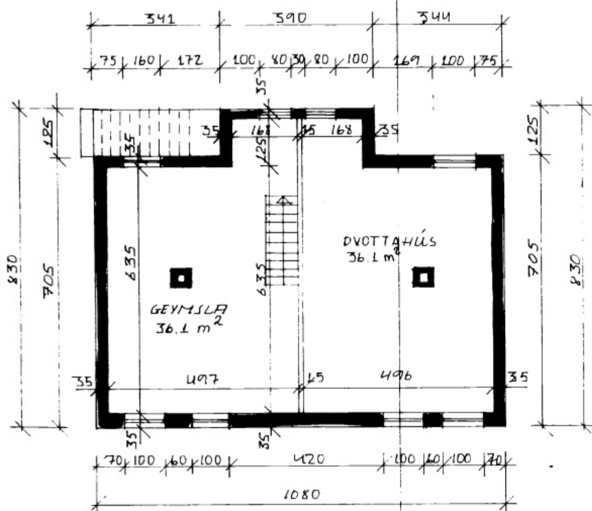
KJALLARI MKV 1:100 A
