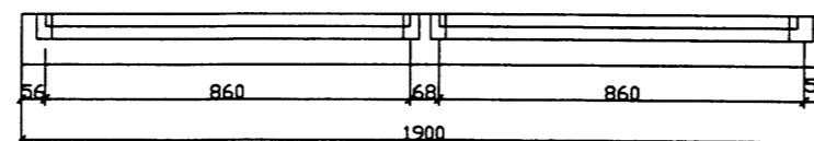
GLUGGI G-2 M=110 2 STK
