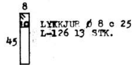
SNID - A 1:20
