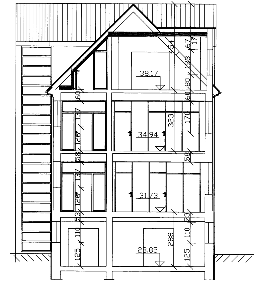
SNID B-B M=1:50
