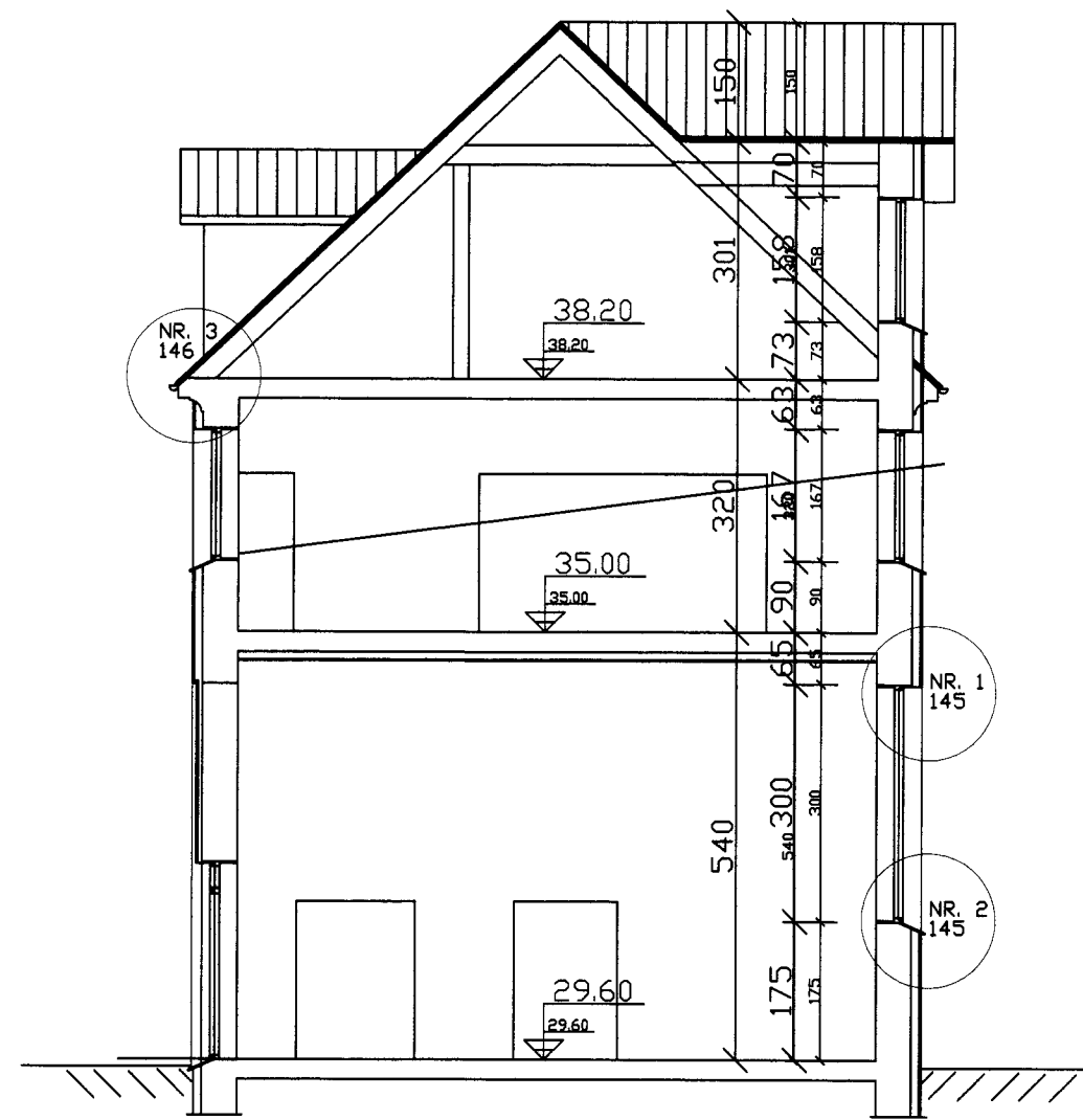
SNID C-C M=1:50
