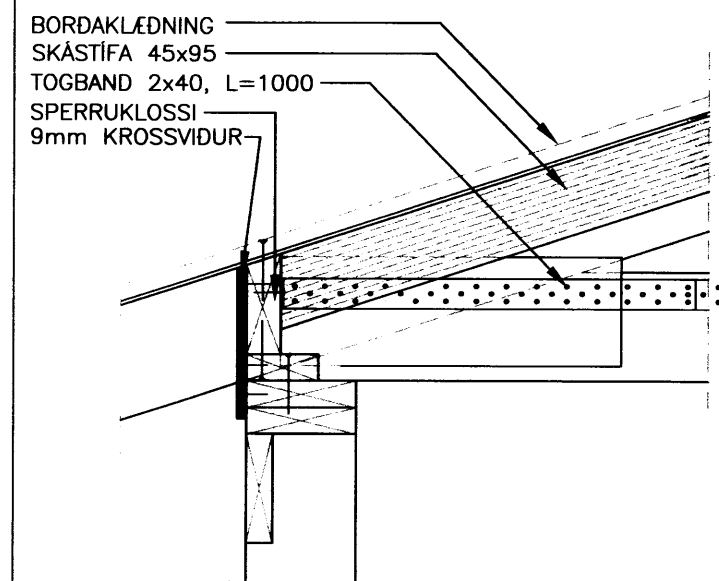
SNID A 1:10
