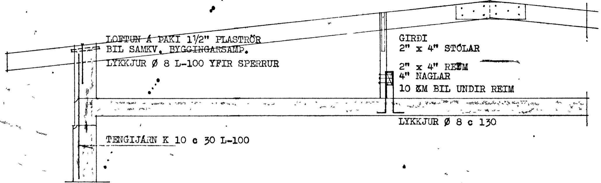
SNID - A 1:20
