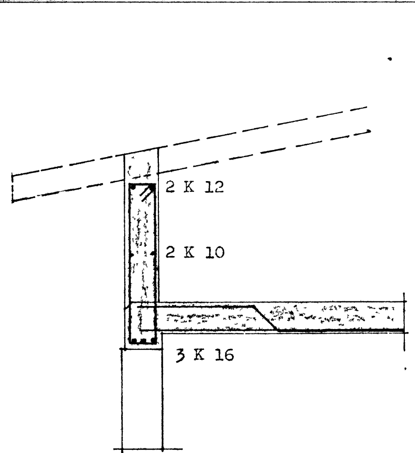
SNID - A 1:20
