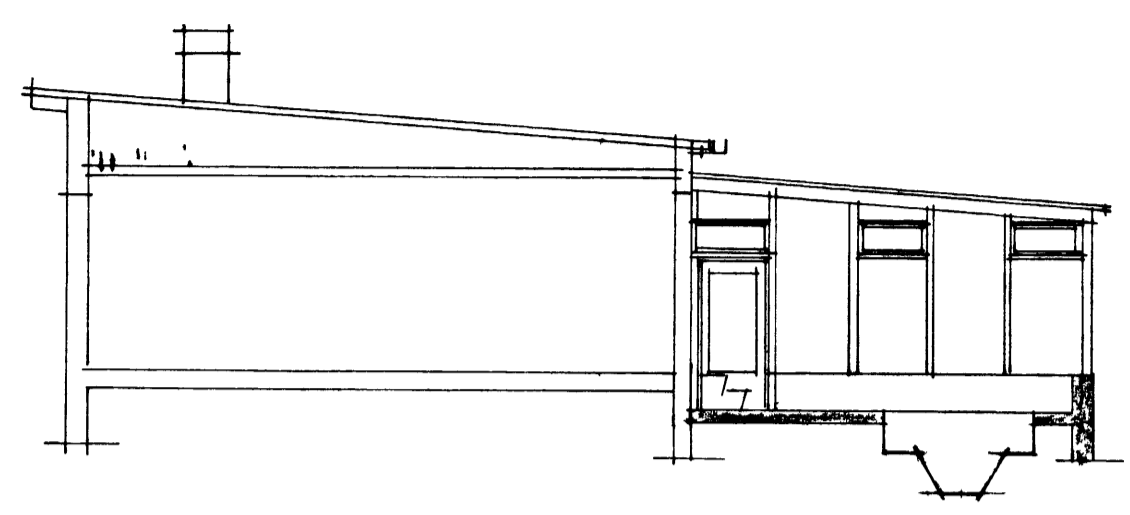
SNIP A-A
