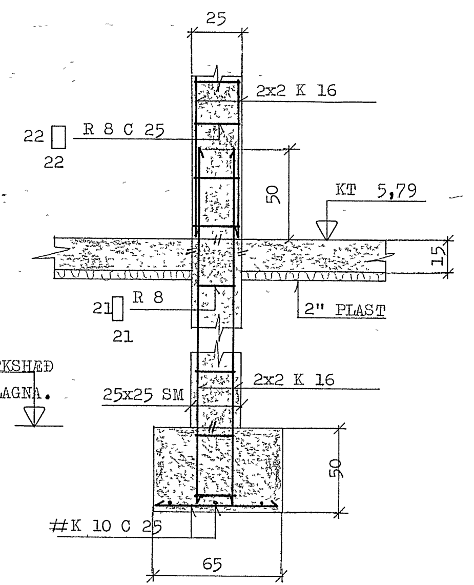
SNID E-E 1:20
