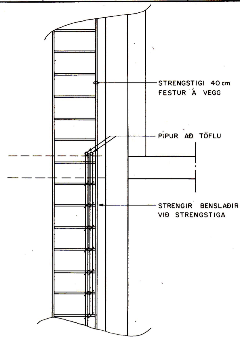
3 SNID M.1:20 4 4
