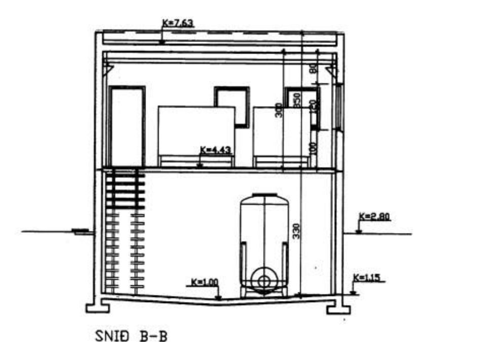
SNID B-B
