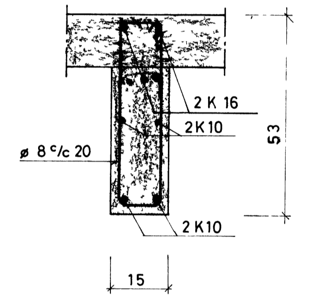
SNID C-C, 1:10
