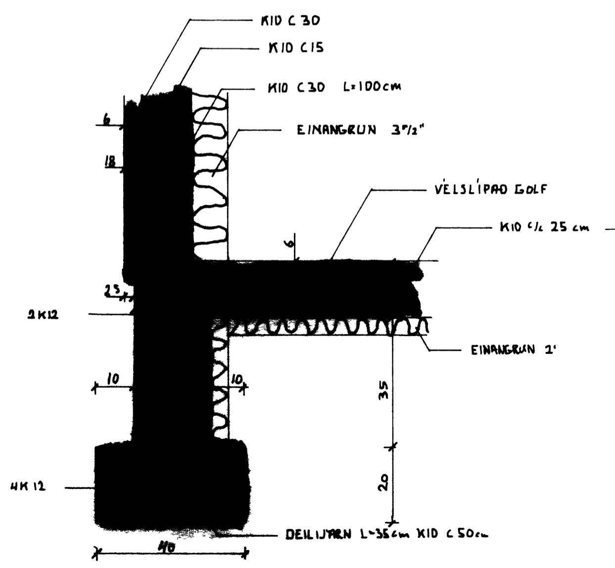
SNID 'I UNDIRST MKV 1-10 A-A
