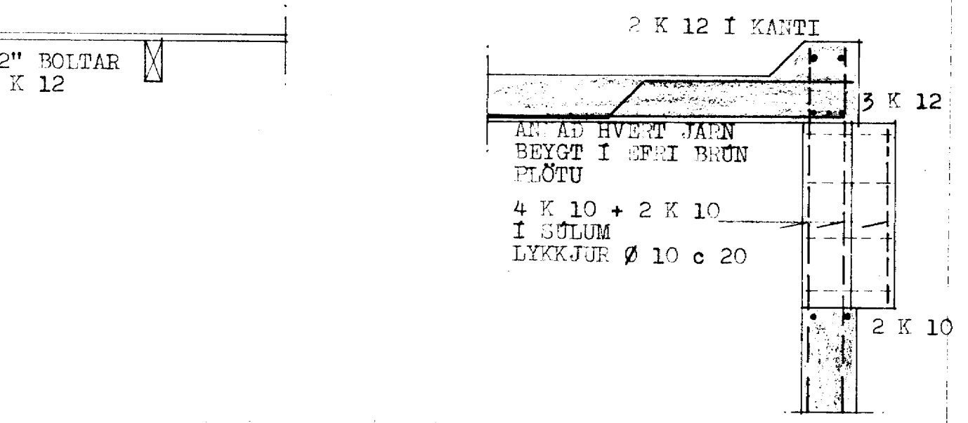
SNID - H 1:20
