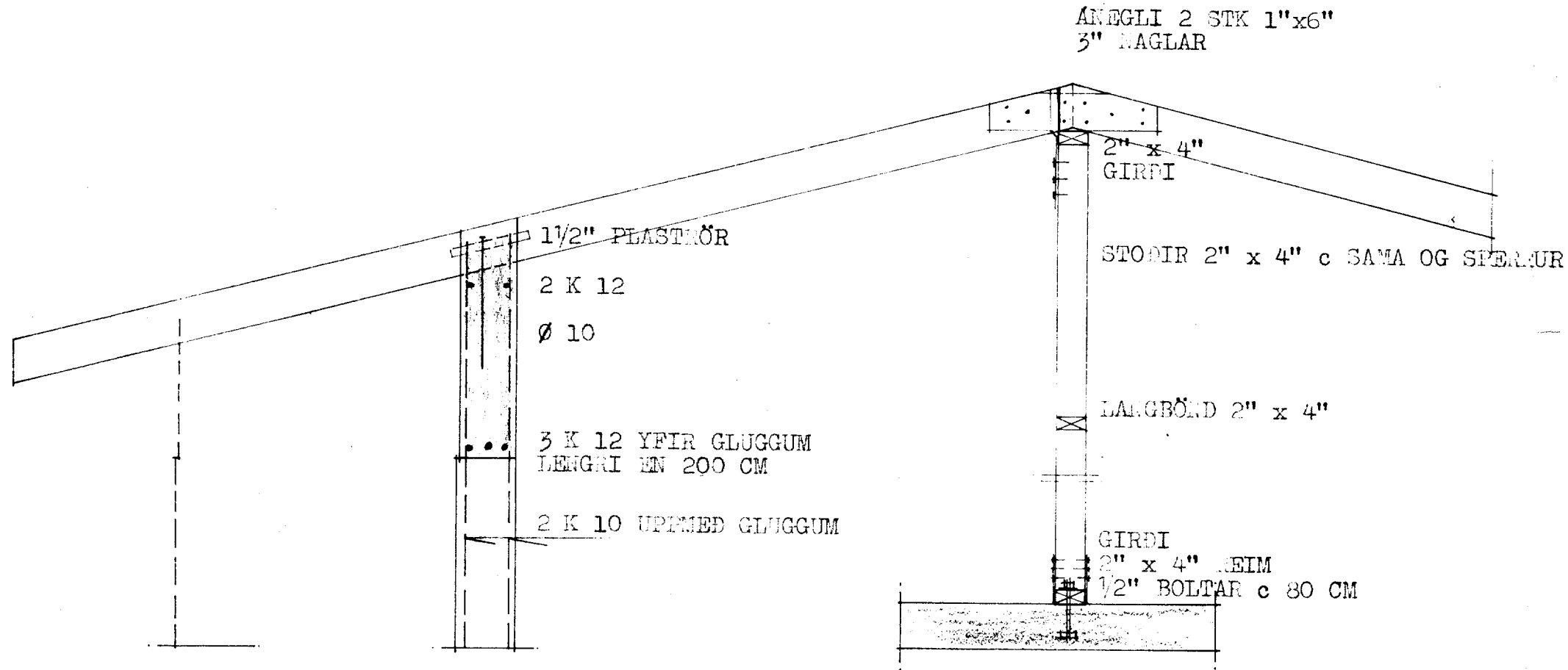
SNID - A 1:20
