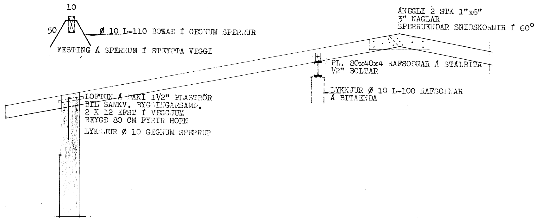
SNID - A 1:20
