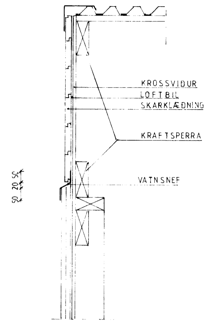
SNID H-H 1:10
