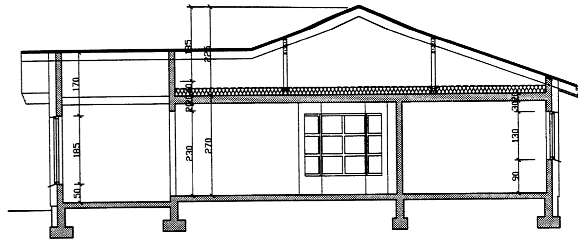
SNID C-C
