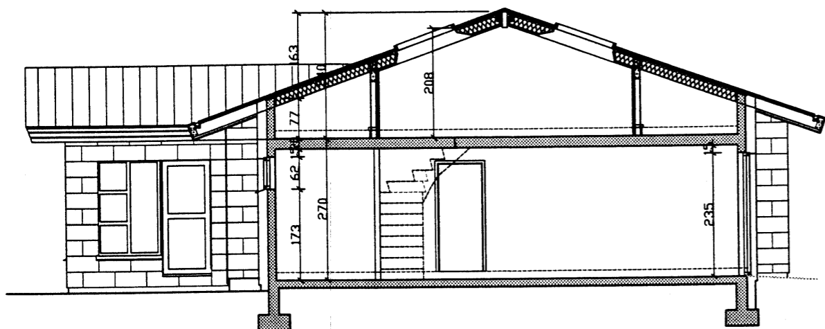
SNID B-B
