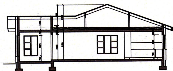
SNID C-C
