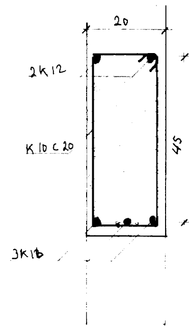
SNID B-B MKV 1:10
