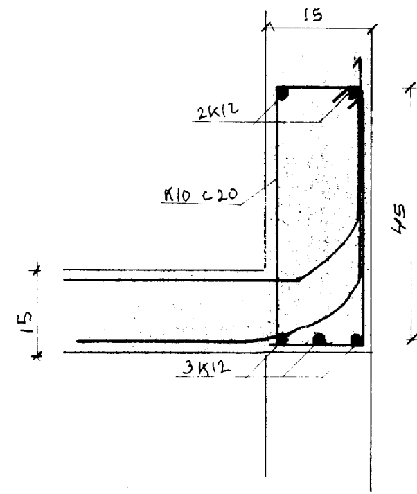
SNID C-C MKV 1:10
