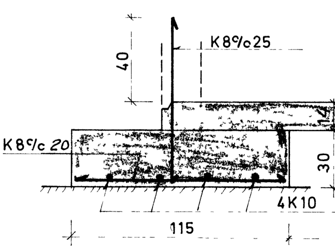
F-F 1 20
