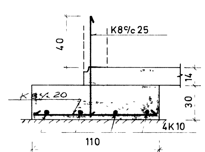
K-K 1 20
