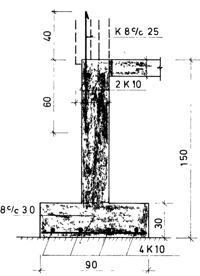
F-F 1 20
