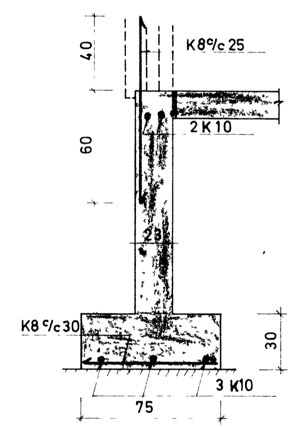
H-H 1 20
