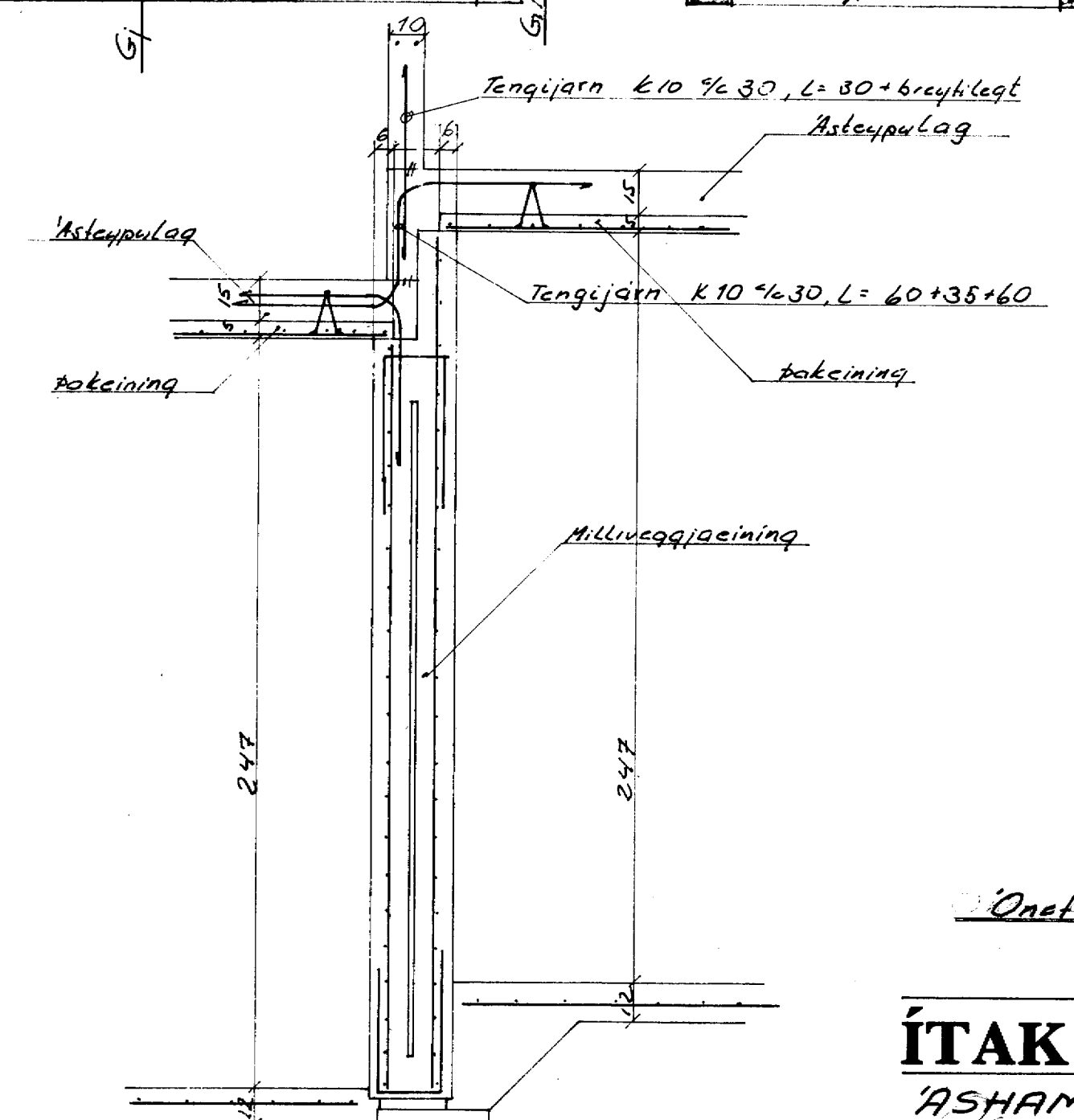
Snid A1: 1:20
